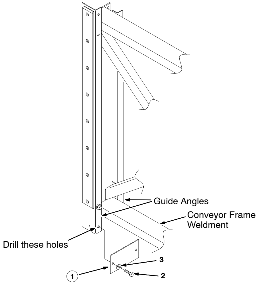
FIG. 1 - Deflector Location
